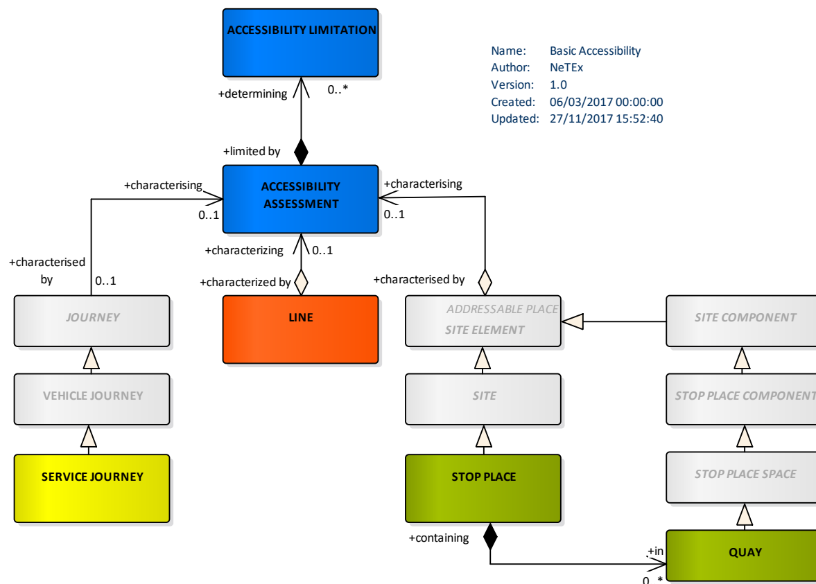
Figure 5 — Accessibility (UML)
